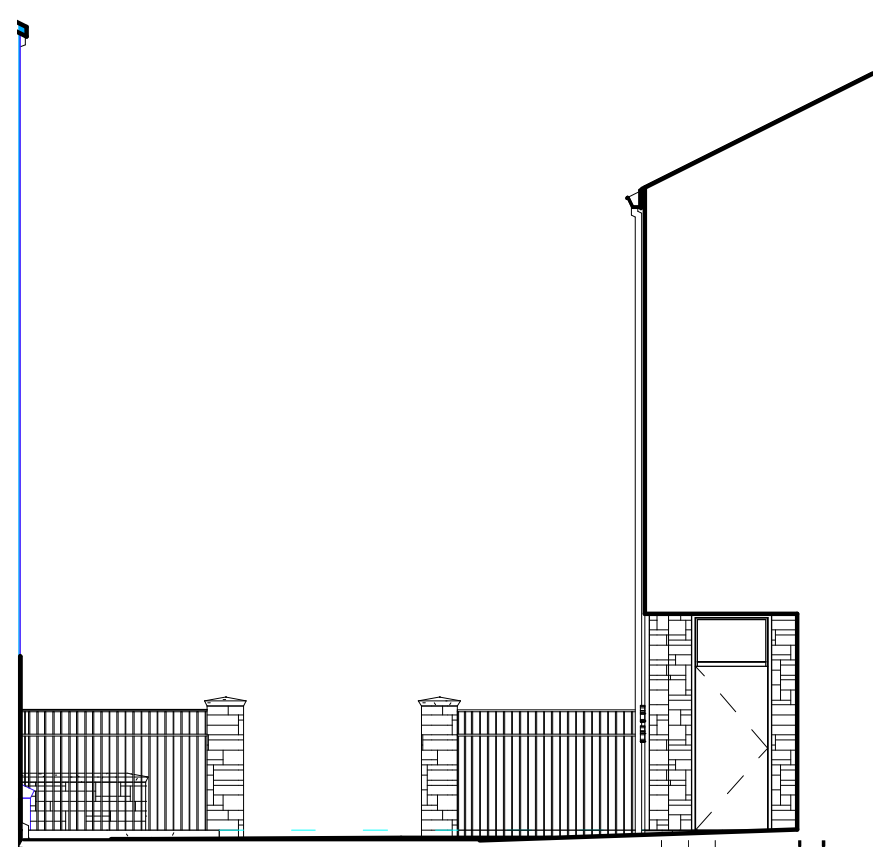
2 COURTYARD ELEVATION - SOUTH 1/8" = 1'-0"
