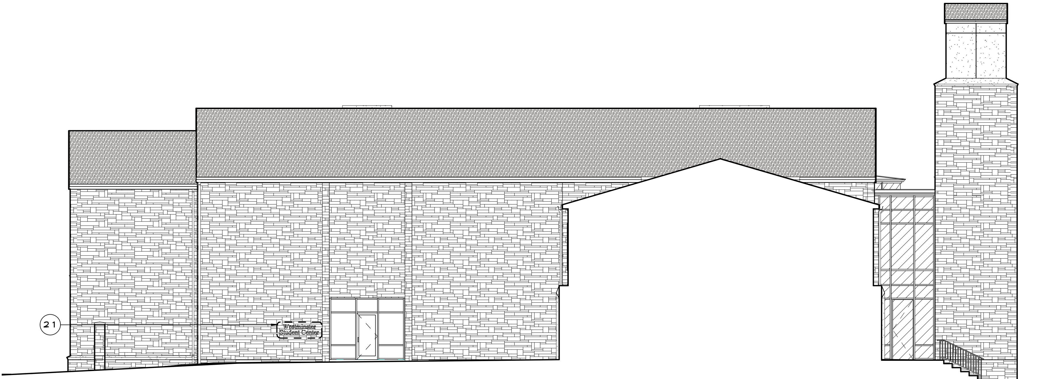
5 COURTYARD ELEVATION - EAST 1/8" = 1'-0"
