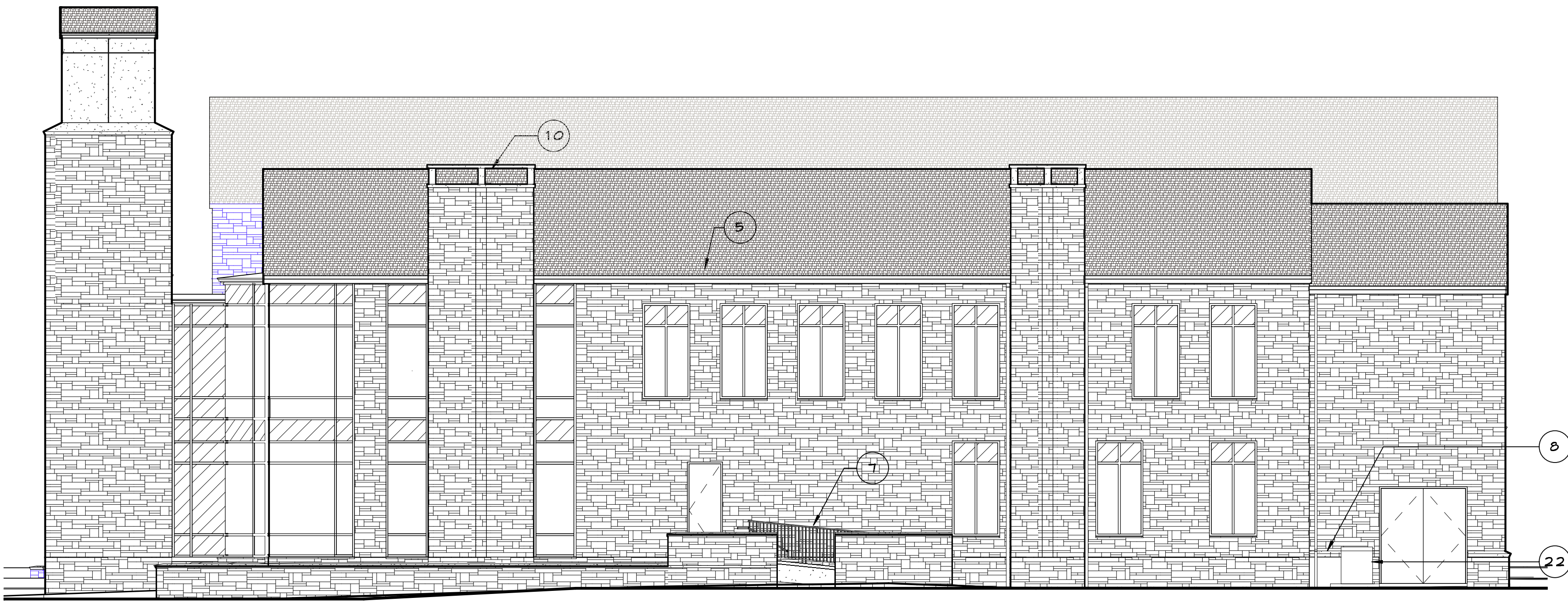
1 WEST ELEVATION 1/8" = 1'-0"
