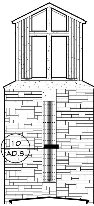
4 BELL TOWER ELEVATION - SOUTH 1/8" = 1'-0"
