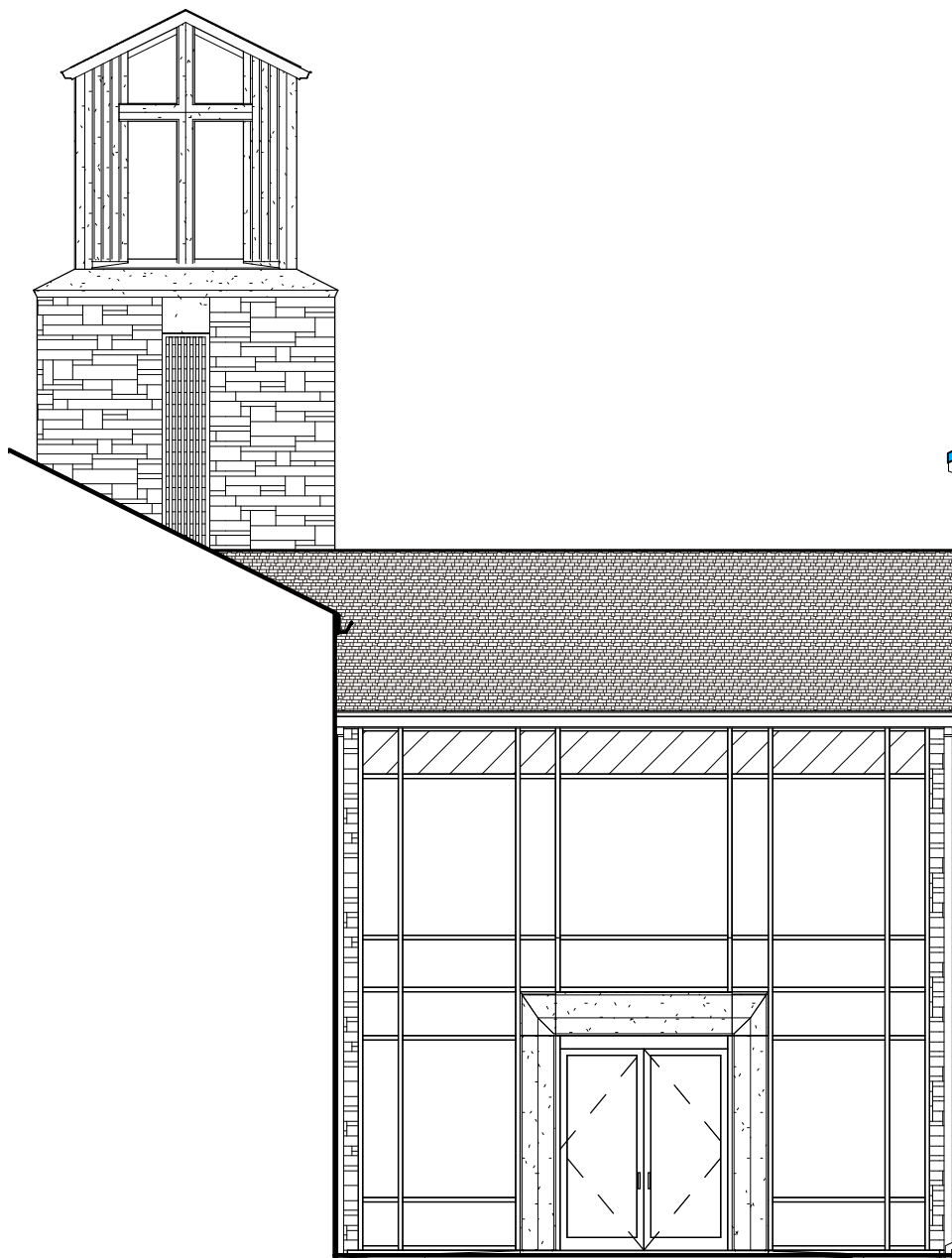
3 COURTYARD ELEVATION - NORTH 1/8" = 1'-0"
