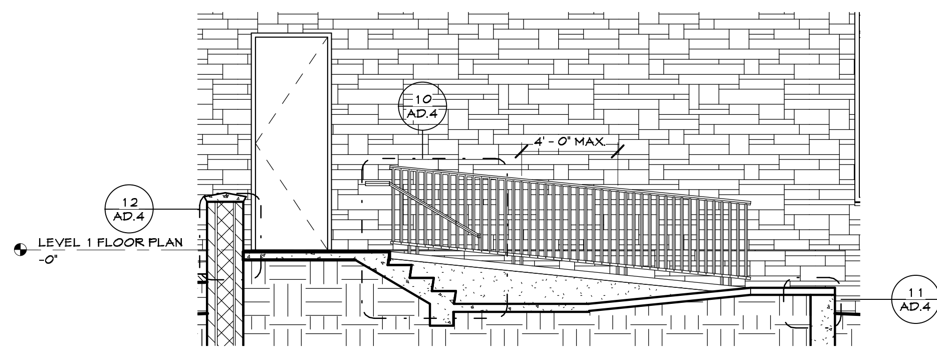
④ LOADING RAMP 1/4" = 1'-0"
