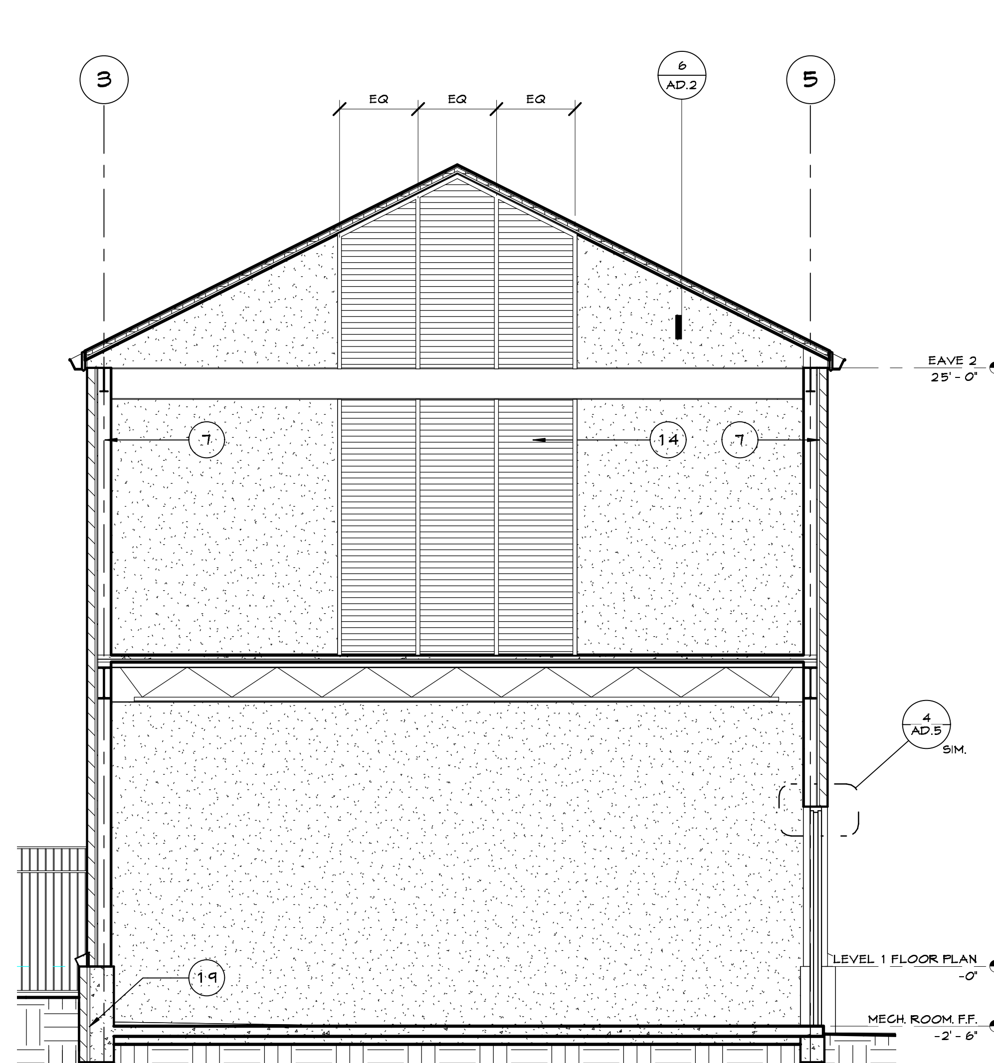
③ MECHANICAL 1/4" = 1'-0"
