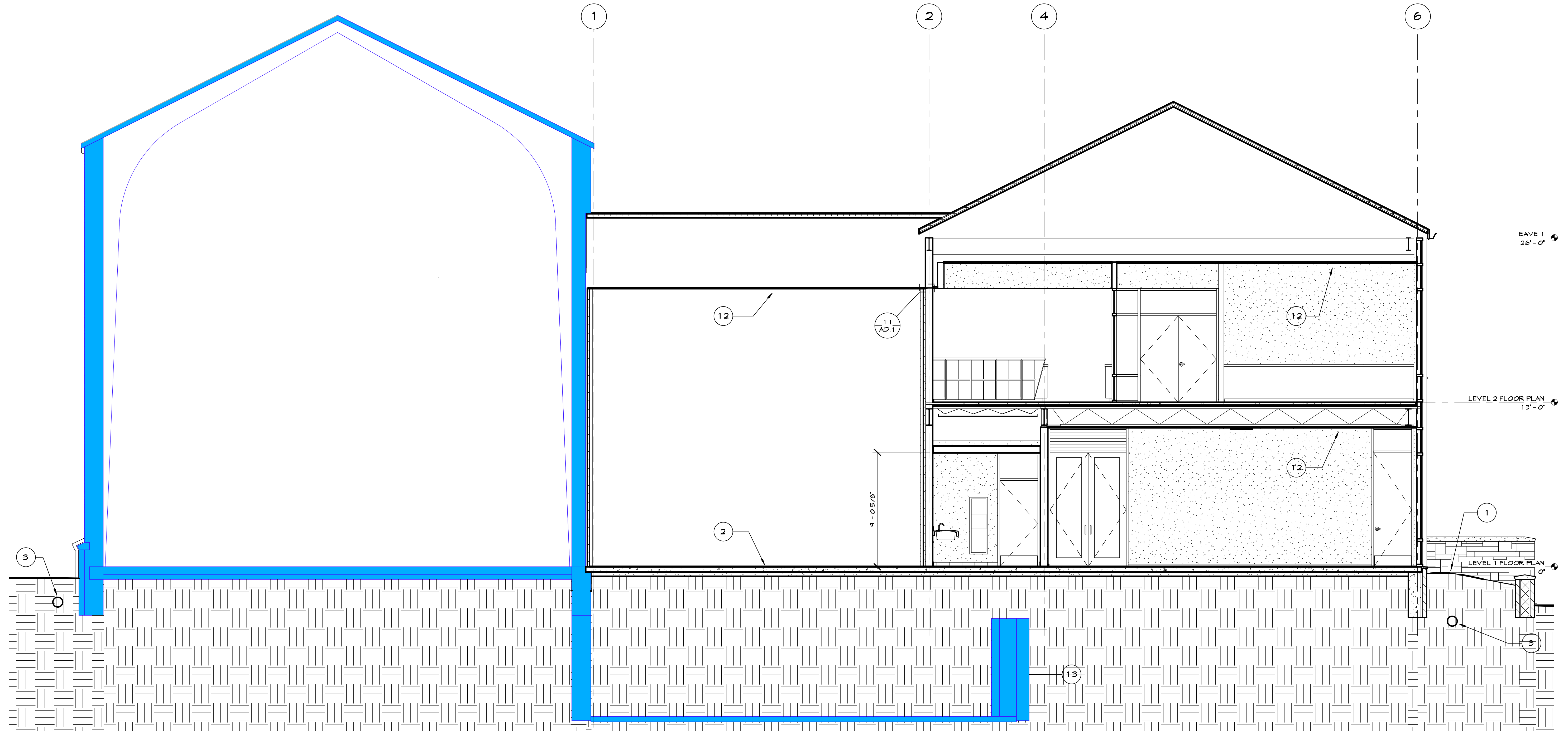
① NAVE/ LOBBY/ RECEPTION 1/4" = 1'-0"
