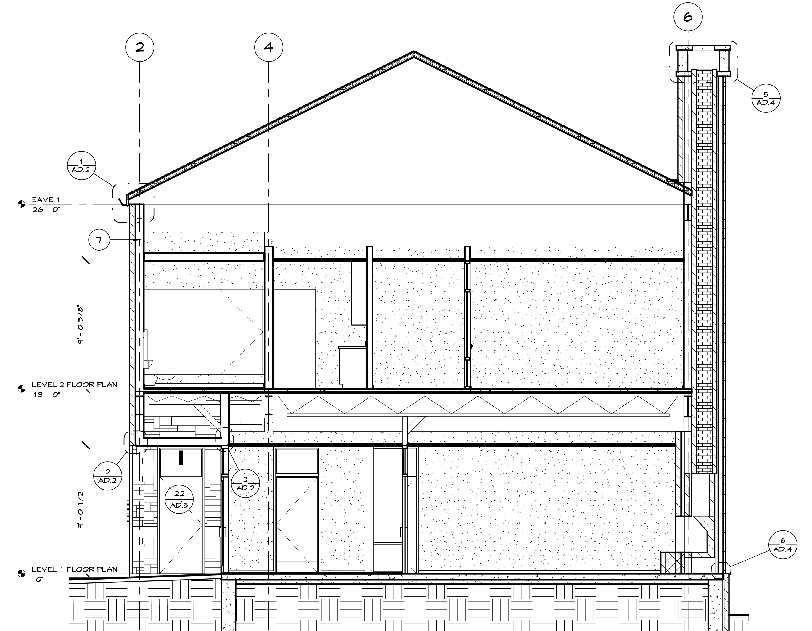
② STUDENT ENTRY/ WESTMINSTER 1/4" = 1'-0"
